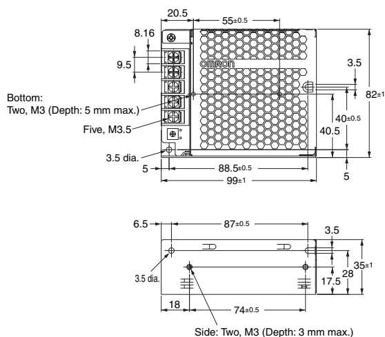
Using the mounting holes in the Power Supply Using the screw holes in the Power Supply Bottom mounting Two, M3 88.5 \pm 0.5 40 \pm 0.5 Two, 3.5 dia. 55 \pm 0.5 Side mounting Two, M3 87 \pm 0.5 Two, 3.5 dia. 74 \pm 0.5
