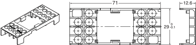
H3Y/H3YN Series for PYFZ-14 PYCZ-C14
