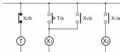
(X): Auxiliary relay such as MY Relay
