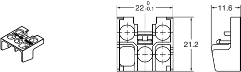
H3Y/H3YN Series for PYFZ-08 PYCZ-C08
