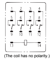
Terminal Arrangement/Internal Connections (Bottom View) Standard Models
