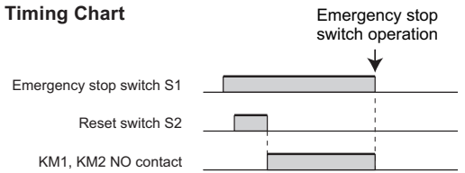
Timing Chart
