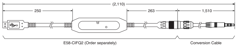
Connected to the E58-CIFQ2 USB-Serial Conversion Cable
