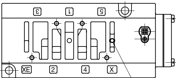
M4 PILOT PORT LOCATION (PLUG #127-691 ORDER SEPARATELY)
